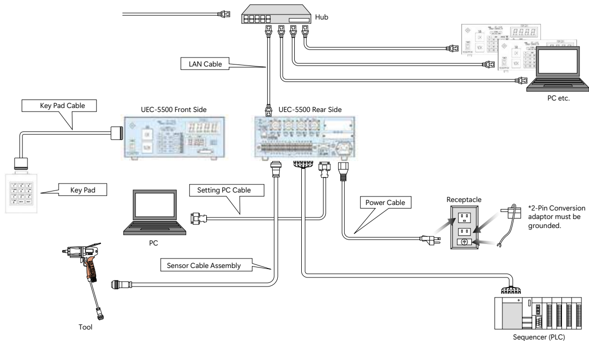
UEC-5500 System Layout
